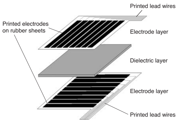
Fig. 1. Schematic structure of smart rubber sensor
