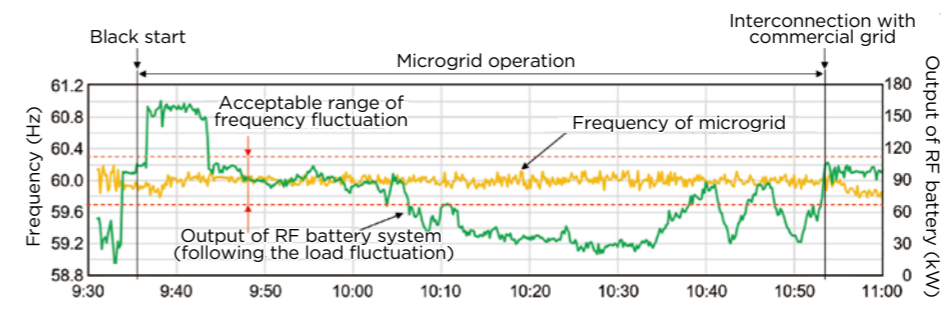
A stable frequency was maintained during microgrid operation. (It is the first time in the U.S. and Japan that a microgrid has been operated on a commercial distribution network inclusive of real consumers with storage batteries as the main power source.)
