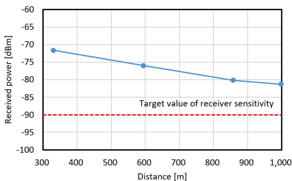
Fig. 7. Distance Characteristic of the Received Signal Strength of Temperature/Current Sensor
